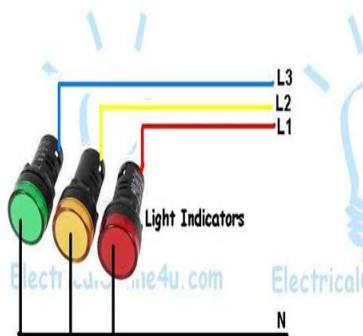
Led Indicator Wiring Diagram for 3 Phase 4 Wire System Design By Sikandar Haidar From ElectricalOnline4u.com
